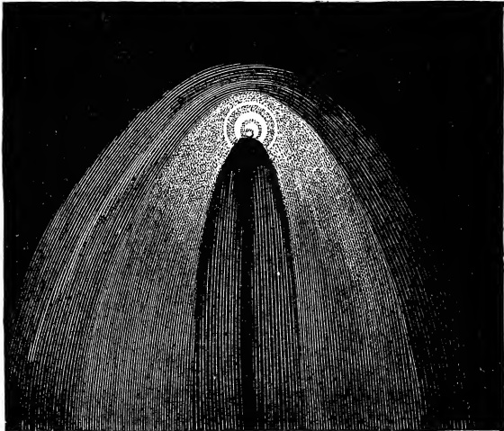
Fig. 74.—How the Tail of a Comet arises.
